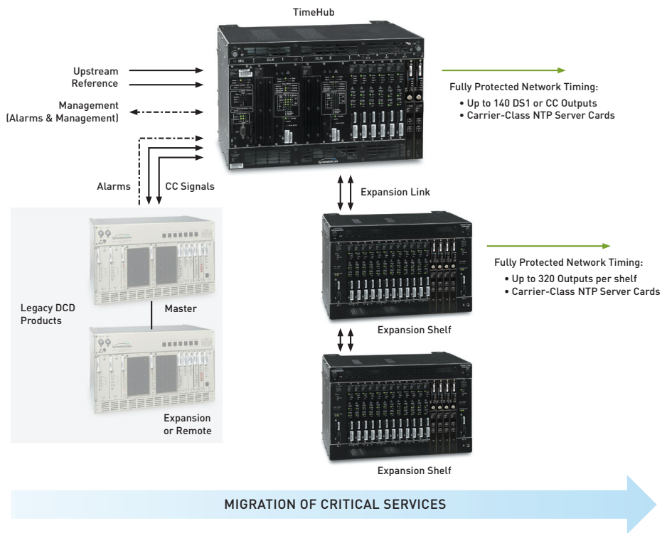
FIG 3: High capacity TimeHub system easily supports NGN network growth, and migration of legacy services.
