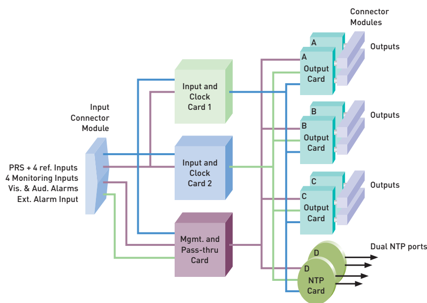
FIG 1: TimeHub 5500 Architecture
