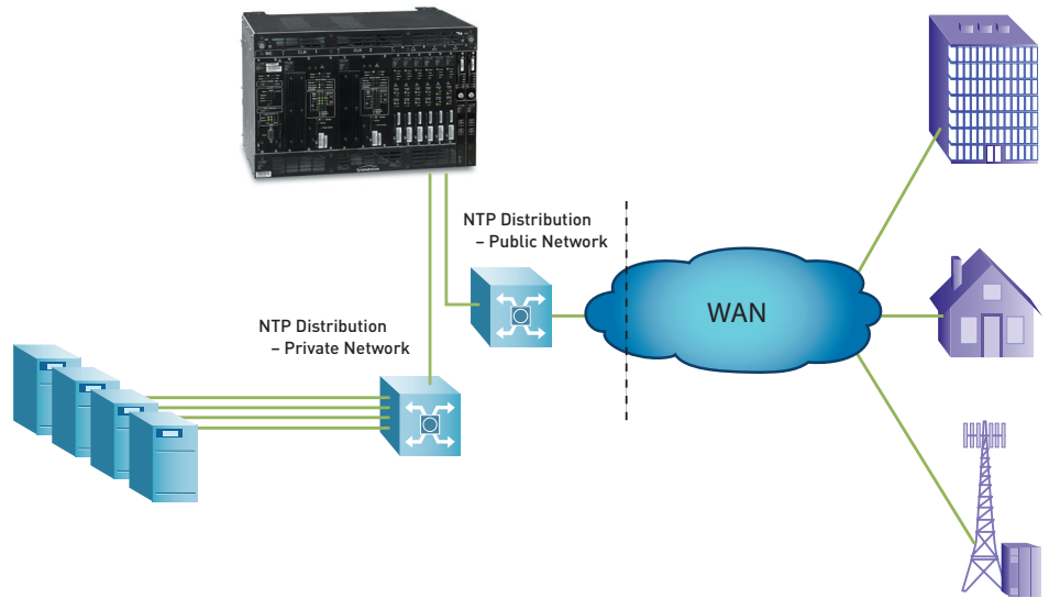
FIG 2: NTP Server cards make it easy to isolate and secure Private network NTP distribution from Public network NTP distribution.
